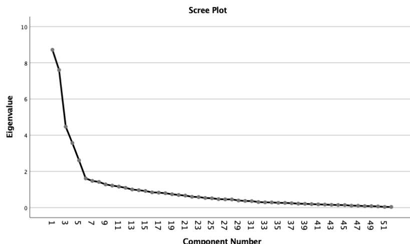
Figure 1. Scree Plot
